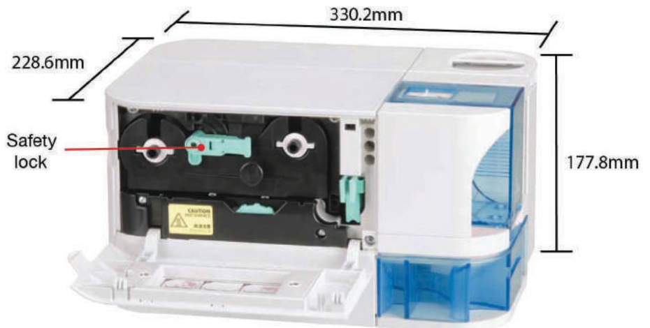
All-in-one removable ribbon cartridge with cleaning assist roller
